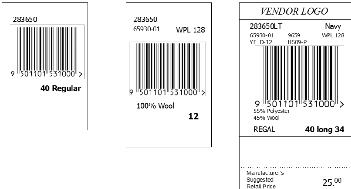
Figure 6.5.3.2-1. Vertical layout
