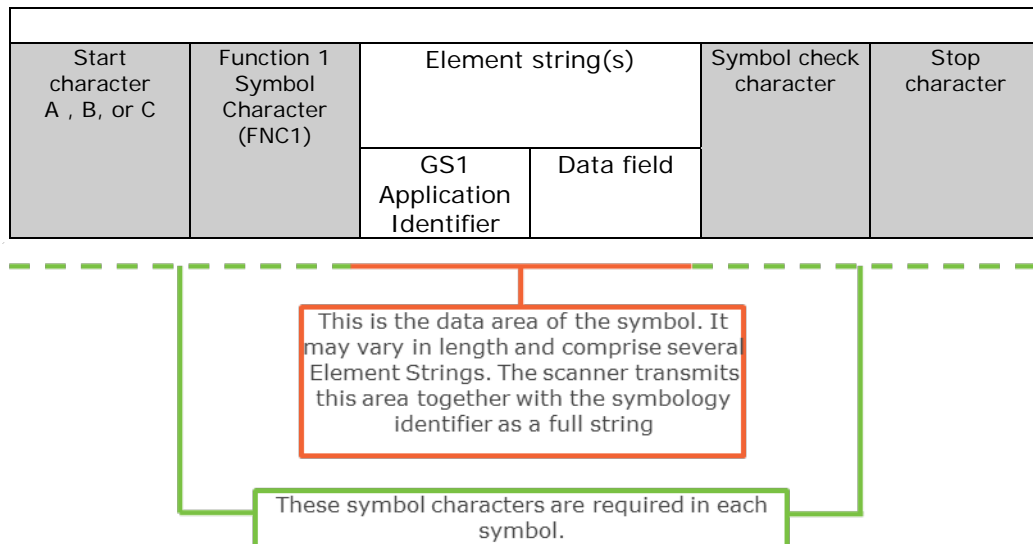
Figure 7.8.5-1. Example GS1-128 barcode structure
